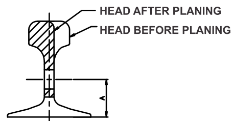
SECTION AT P & S
