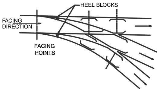
THREE THROW SWITCH (SIMILAR FLEXURE)
