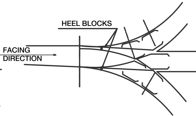
THREE THROW SWITCH (CONTRARY FLEXURE)
