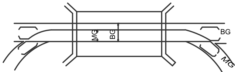
GAUNTLETED TRACK FOR MIXED GAUGE
