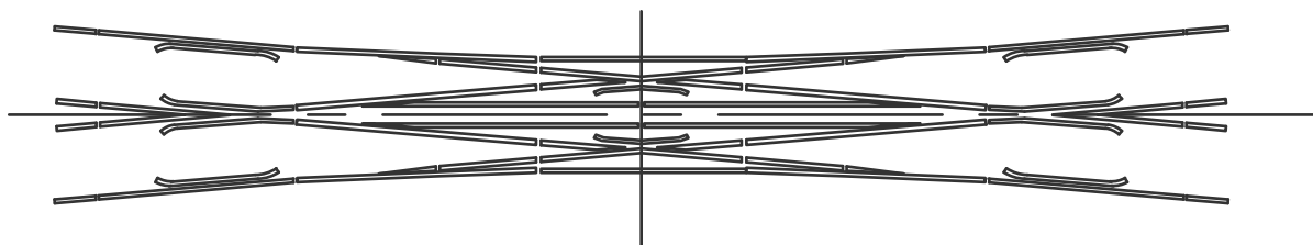
DIAMOND CROSSING WITH DOUBLE SLIP
