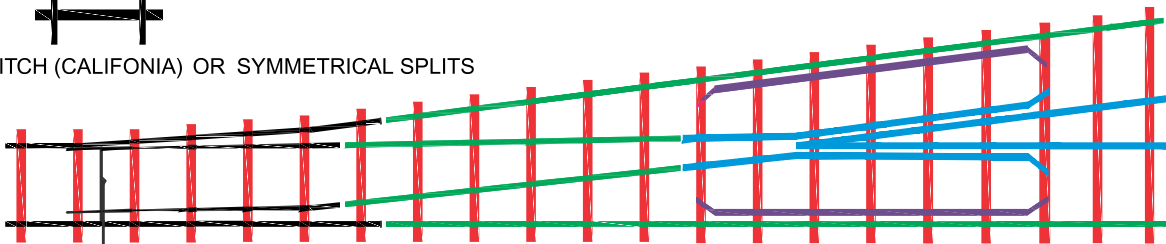
6) COMPLETE TURNOUT FITTINGS
