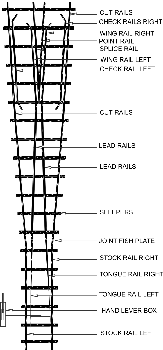
'Y' SWITCH (CALIFONIA) OR SYMMETRICAL SPLITS
